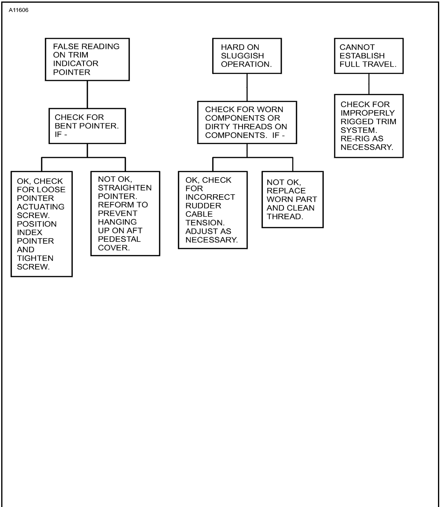
Figure 101 : Sheet 1 : Rudder Trim System Troubleshooting Chart
